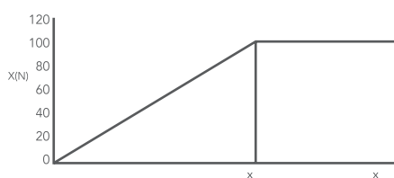
Figure 2 Standardzation with minimum objective
