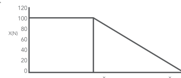
Figure 3 Maximum objective standardization
