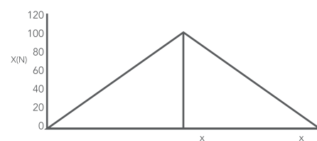
Figure 4 Single objective standardization
